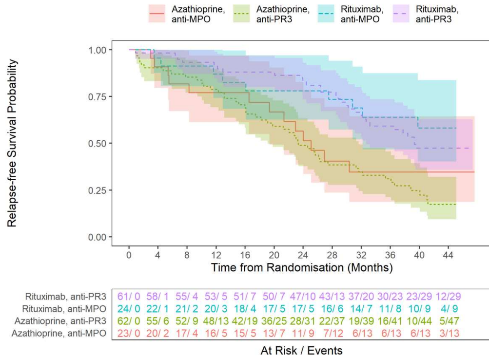
Supplementary Figure 1: Probability of relapse-free survival: rituximab compared to azathioprine according to ANCA sub-type: anti-MPO or anti-PR3
