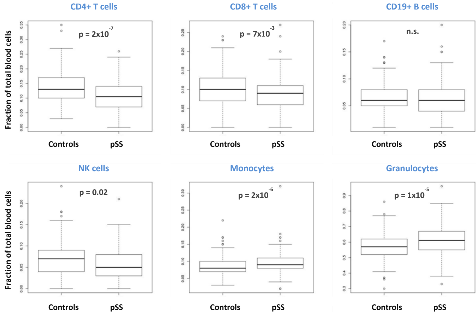
Supplementary figure S1. Differential blood cell type estimates for control individuals and patients with primary Sjögren's syndrome (pSS). Boxplots illustrating the estimated cell type fractions in whole blood samples from controls and patients with pSS for CD4+ T cells, CD8+ T cells, CD19+ B cells, natural killer (NK) cells, monocytes and granulocytes.
