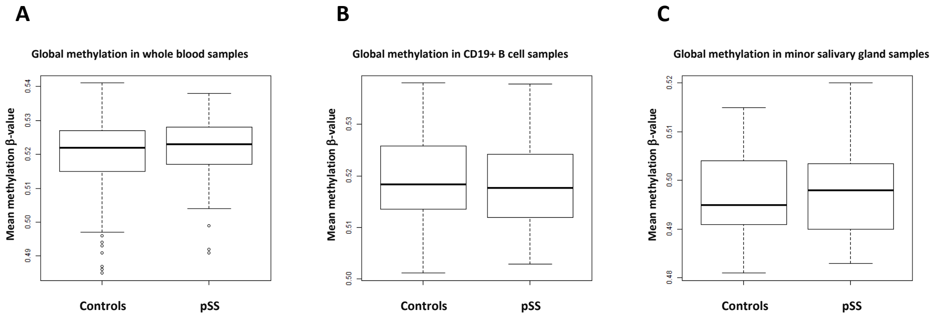
Supplementary figure S2. Global methylation across all analyzed sites in whole blood, CD19+ B cell and minor salivary gland biopsy samples from control individuals and patients with primary Sjögren's syndrome (pSS). Boxplots illustrating the mean methylation \beta (beta)-value across all analyzed CpG sites per sample for controls and patients with pSS, (A) in whole blood, (B) in CD19+ B cells and (C) in minor salivary gland biopsies.
