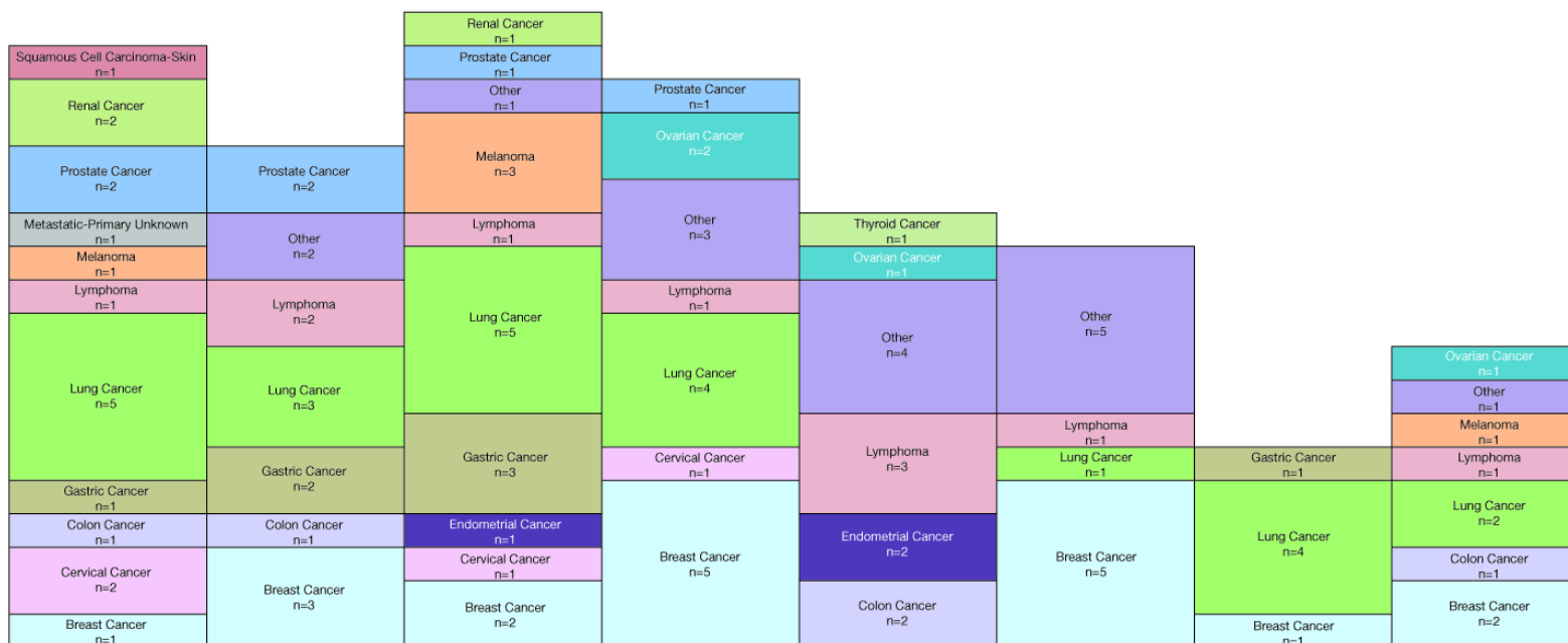
Online Supplemental Appendix Figure 2. Each malignancy (excluding non-melanoma skin cancer)* in tofacitinib-treated patients observed per 6-month intervals†
