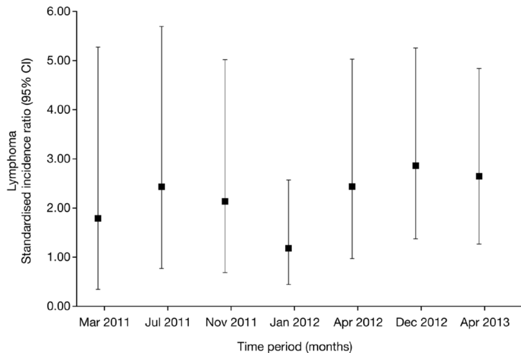
Online Supplemental Appendix Figure 1. Age-and-sex-adjusted standardised incidence ratios (95% CI) (SEER referent) for lymphoma with increasing tofacitinib exposure over time
