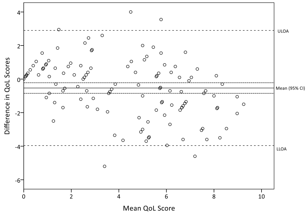
Supplementary Figure 13. Bland-Altman plot of difference in QoL scores
