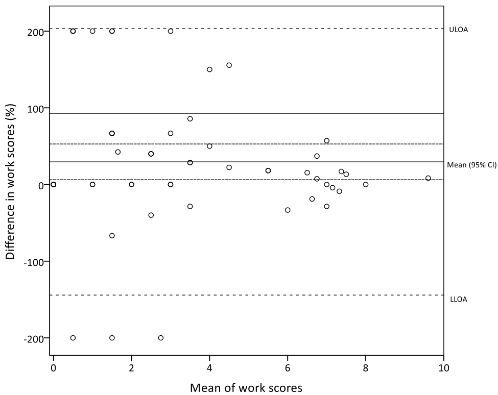
Supplementary Figure 9. Bland-Altman plot of percentage difference in work scores (Presenteeism and Impairment combined)
