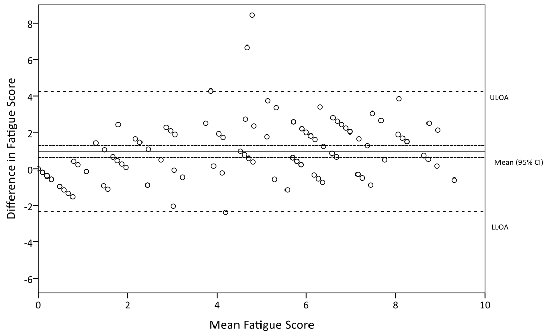
Supplementary Figure 4. Bland-Altman plot of difference in Fatigue scores
