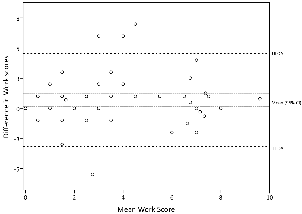
Supplementary Figure 8. Bland-Altman plot of difference in work scores (Presenteeism and Impairment combined)
