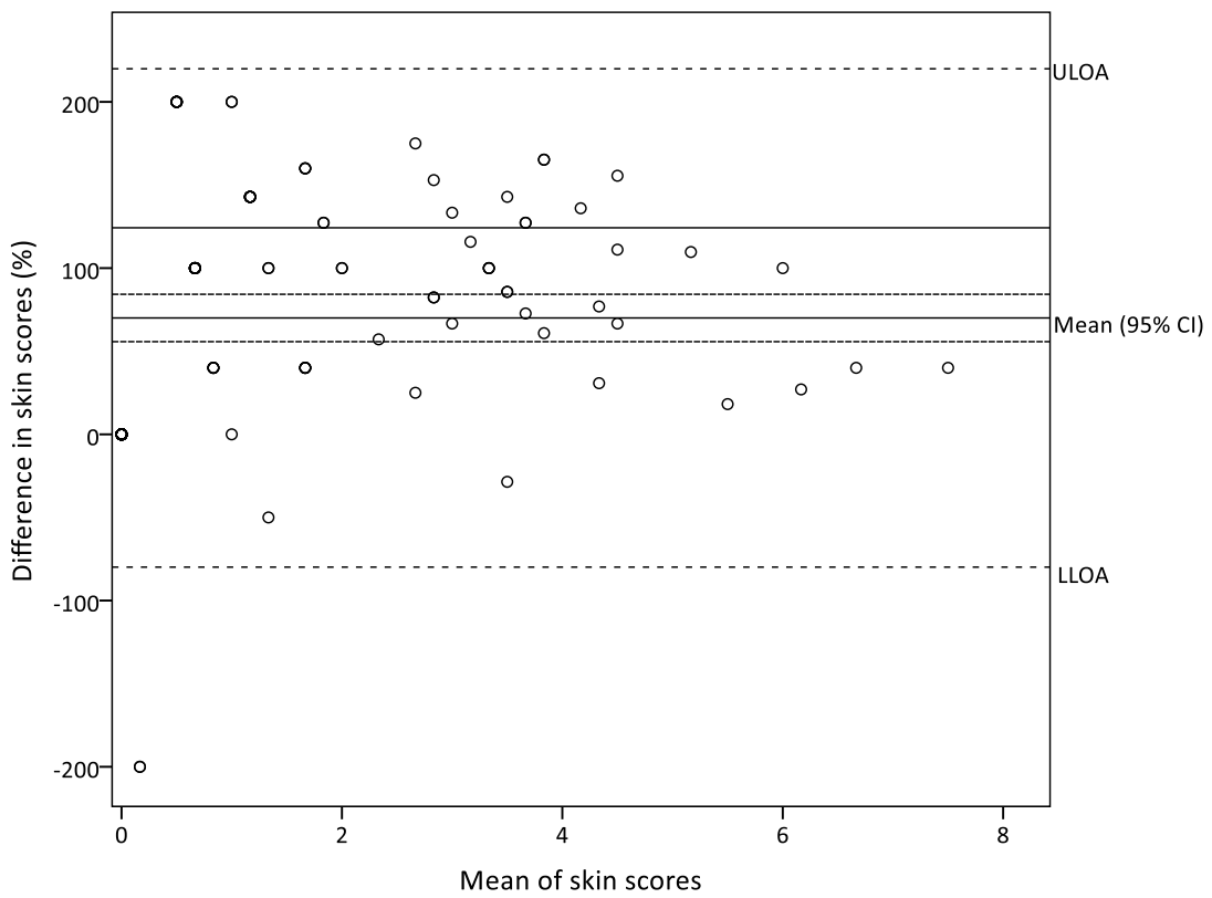
Supplementary Figure 7. Bland-Altman plot of percentage difference in skin scores
