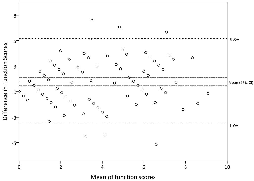
Supplementary Figure 11. Bland-Altman plot of differences in function scores
