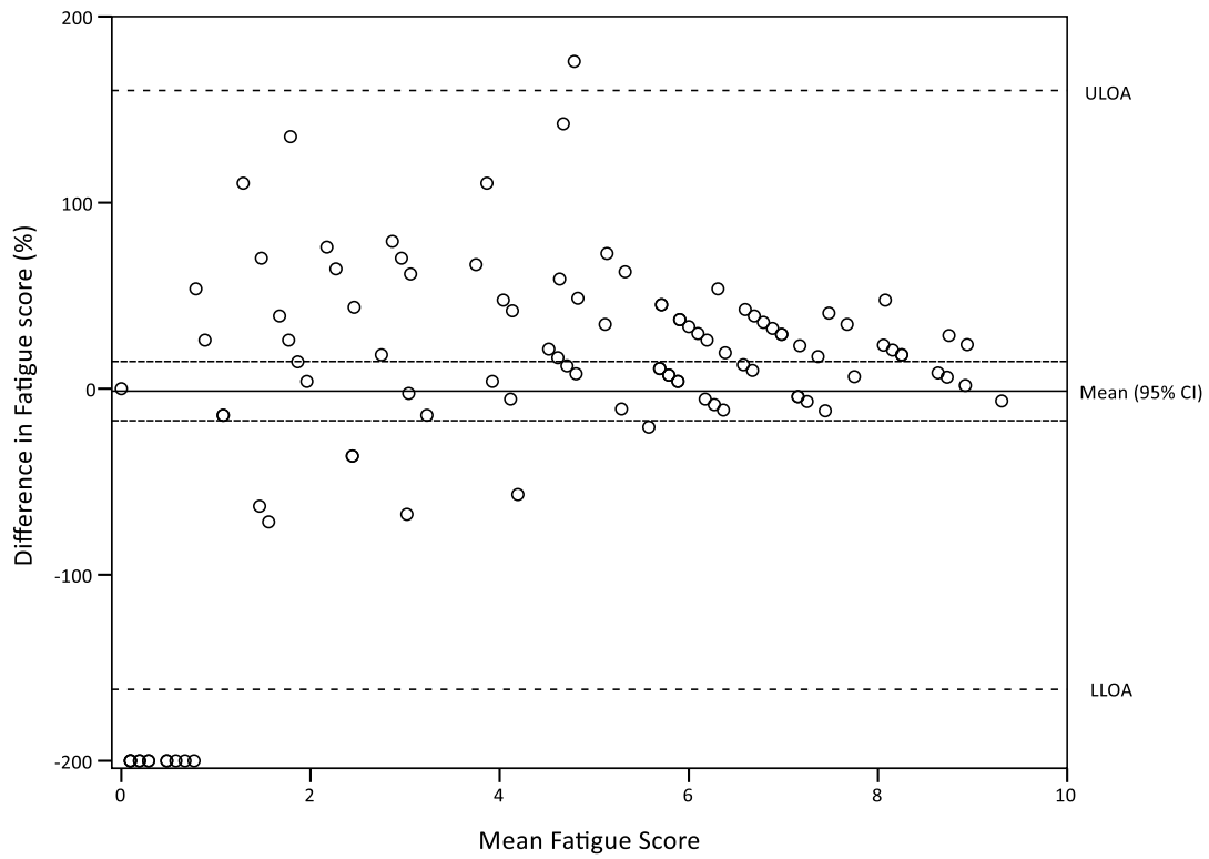
Supplementary Figure 5. Bland-Altman plot of percentage difference in Fatigue scores
