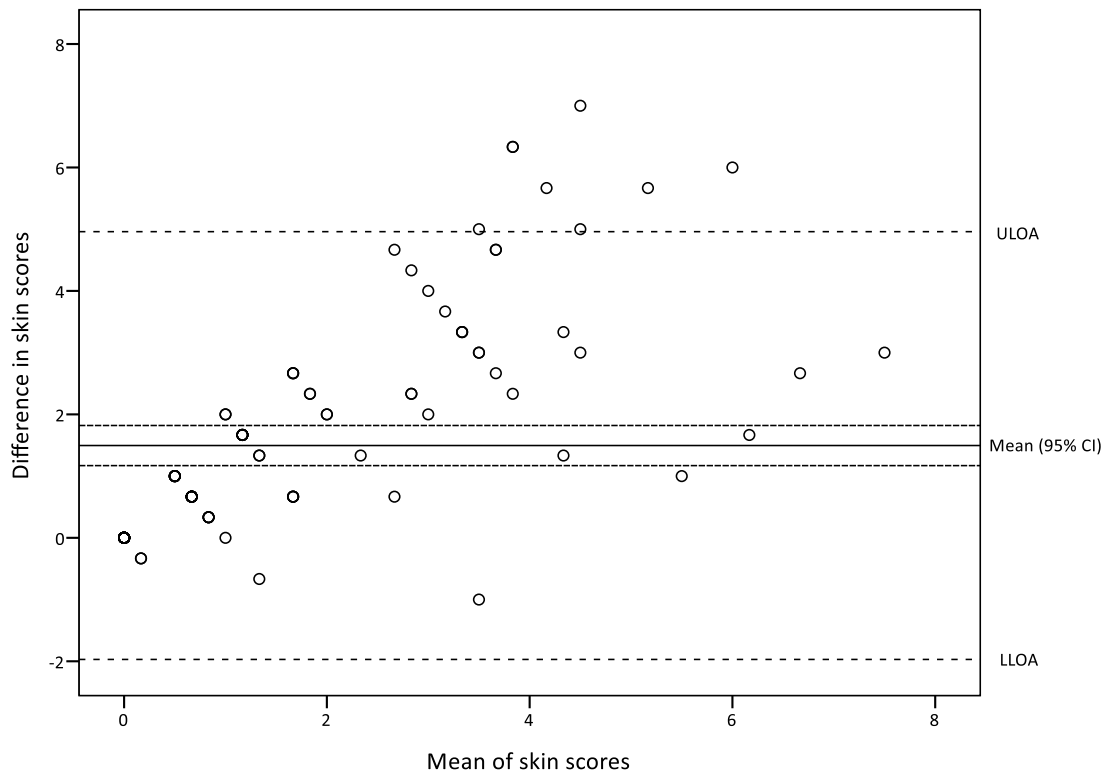
Supplementary Figure 6. Bland-Altman plot of difference in skin scores
