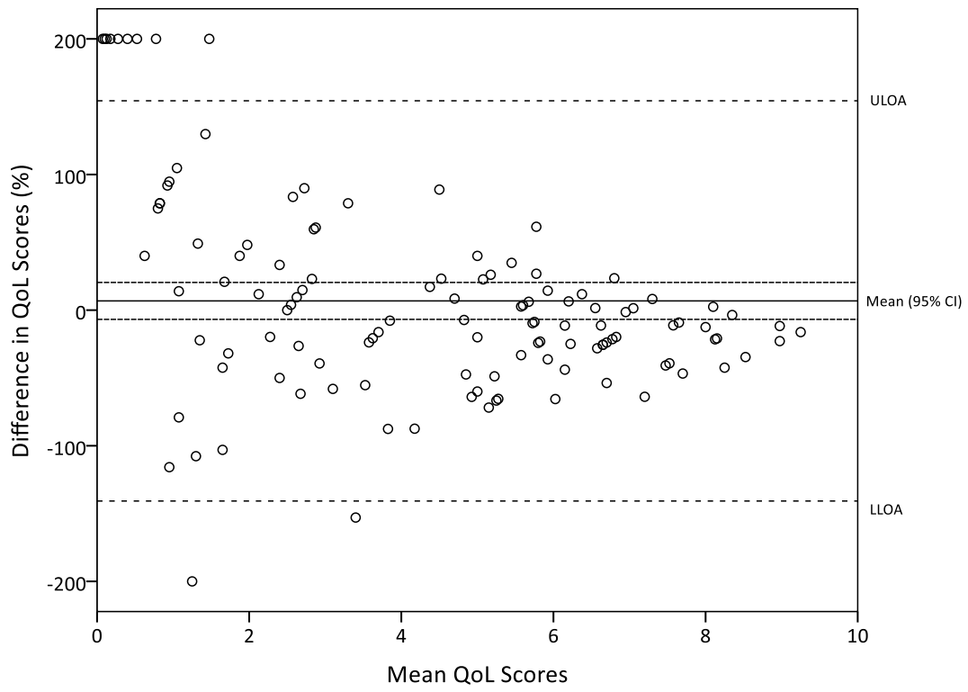
Supplementary Figure 14. Bland-Altman plot of percentage difference in QoL scores
