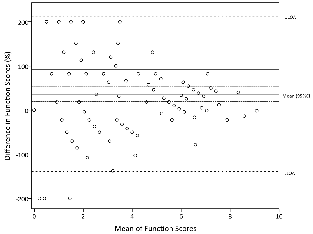
Supplementary Figure 12. Bland-Altman plot of percentage difference in function scores
