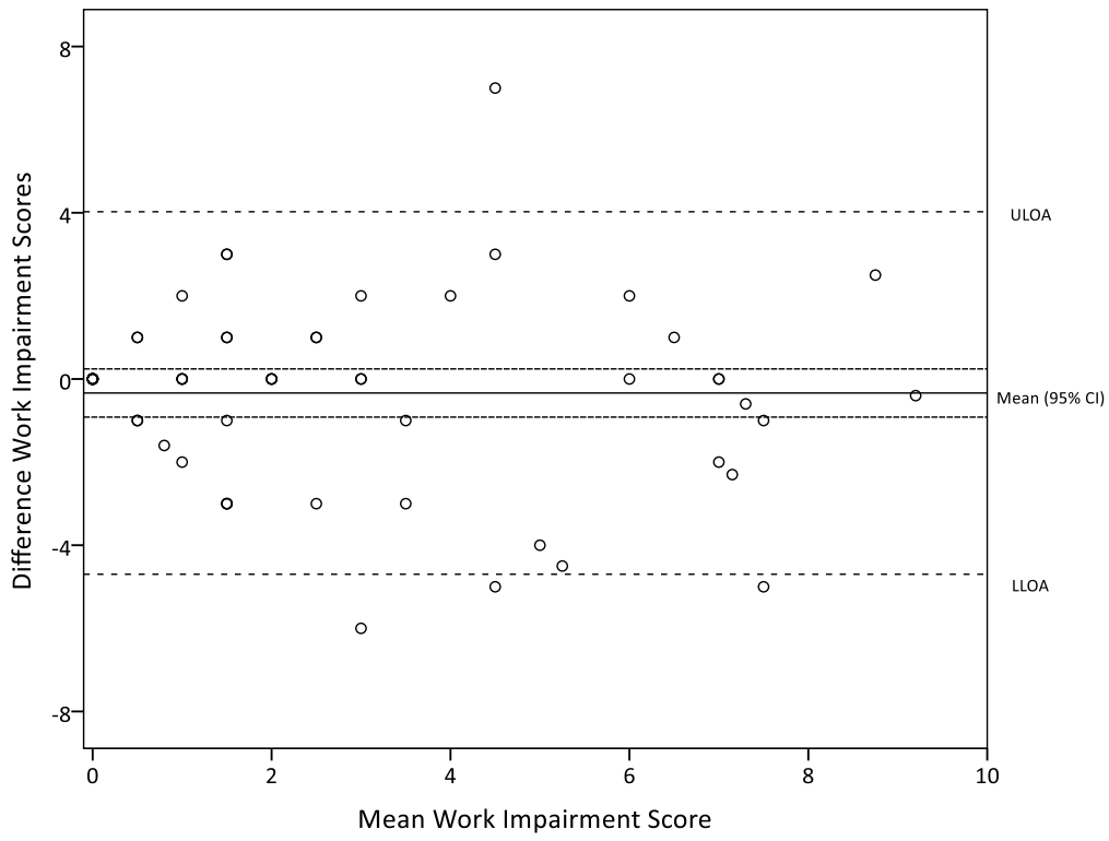
Supplementary Figure 10. Bland-Altman plot of differences in work impairment scores
