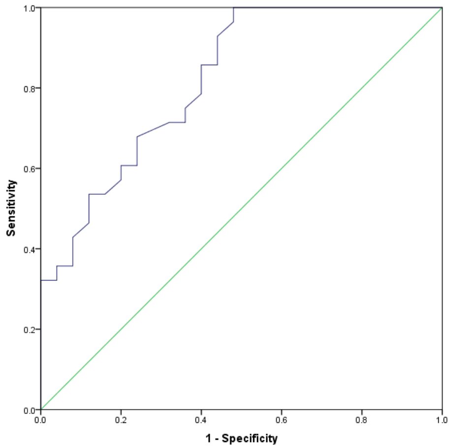
Supplementary Figure 3. Receiver operating characteristic curve showing absolute change in psoriatic arthritis impact of disease (PsAID) score at 3 months.
