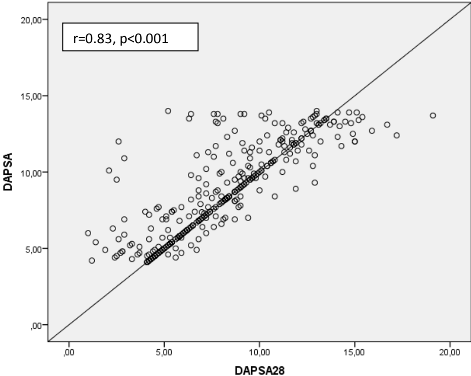
Supplementary Figure S2b Scatterplot of baseline DAPSA and DAPSA28 for patients in DAPSA low disease activity (n=342)
