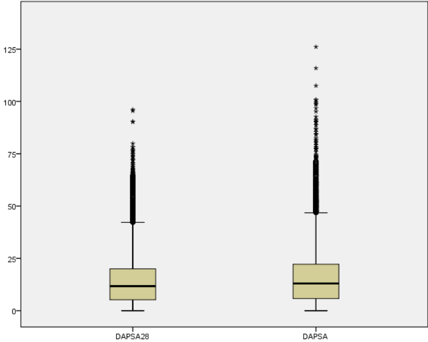
Supplementary figure S1 Boxplot of DAPSA and DAPSA28 (all visits, n=6421)
