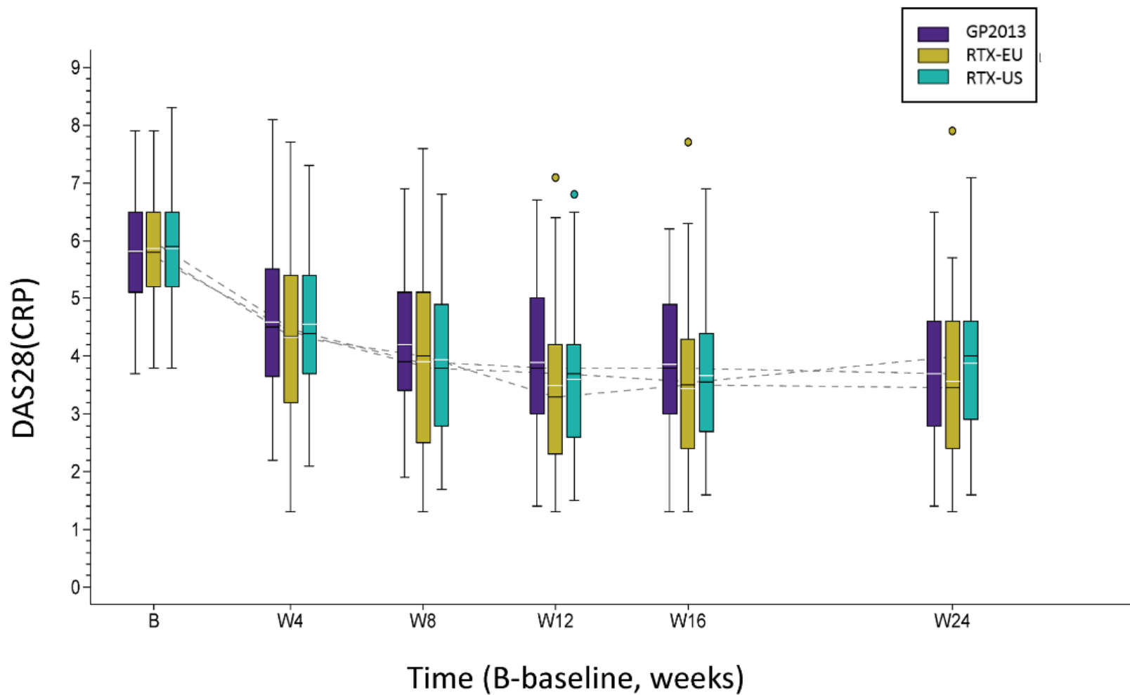
Figure S3. Panel A: Box whisker plot of DAS28(CRP) for the GP2013, the RTX-EU and RTX-US treatments arms (Per Protocol Set)
