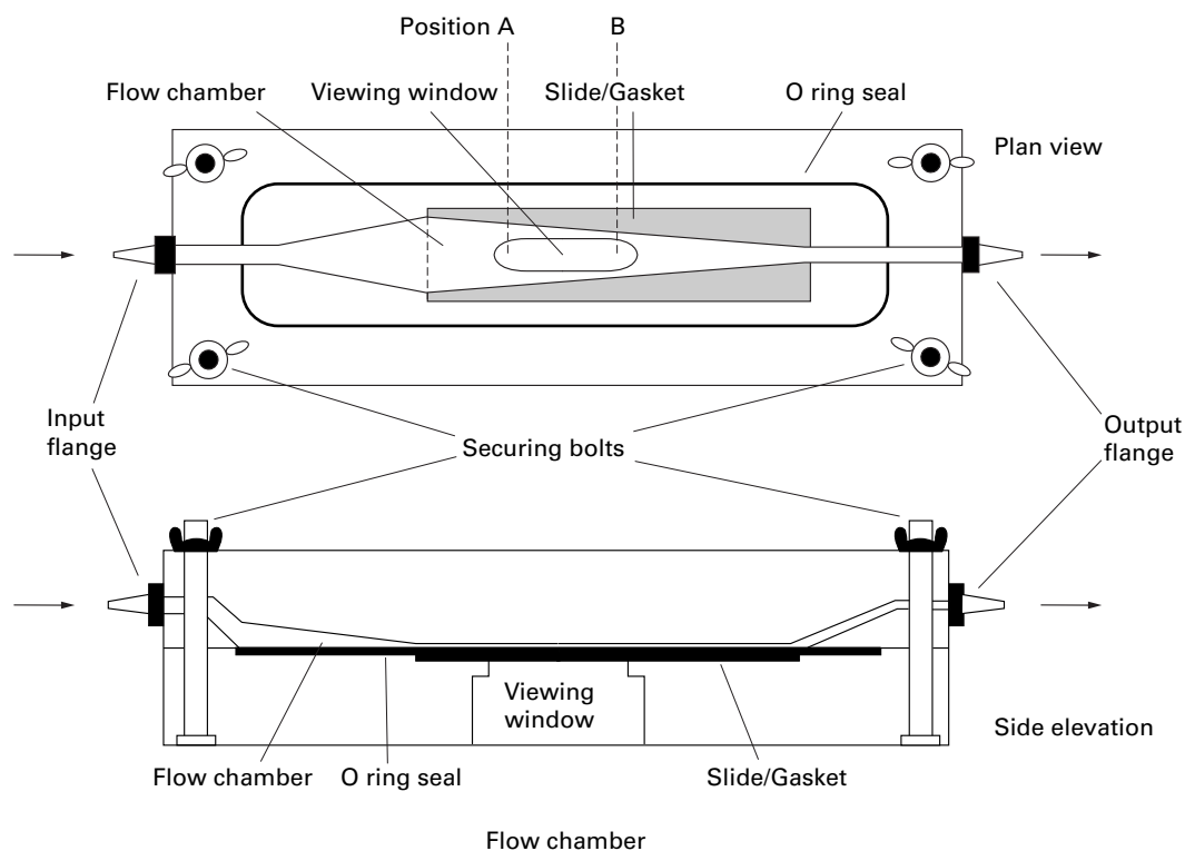
Figure 1 Schematic representation of the parallel plate flow cell used. The convergence of the side walls of the cell increases the velocity of the perfusate as it travels through the cell. This increase in velocity permits measurements to be made on cells exposed to an increasing wall shear stress in the same system without changing the mass flow volume. Wall shear stress at position A ( \tau_A ) = 2.4 dynes/cm 2 and \tau_B = 4.0 dynes/cm 2 assuming a volumetric flow rate of 0.916 cm 3 /sec (55 ml/min).
